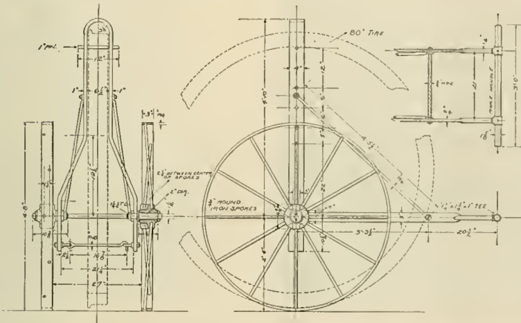
DETAILS OF TIRE TRUCK.
